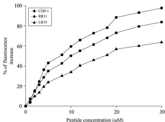
Fig. 3. Plot showing changes in fluorescence intensity of FITC of FITC-LPS, in terms of percentage normalized with respect to Triton-X100, as a function of concentrations of CDP-1, RR11 and LR10 peptides. Fluorescence experiments were performed at 10 mM sodium phosphate buffer, pH 7.0. The excitation of FITC was set to 480 nm and emission was collected from 500 to 550 nm. All lines along the data points are for guiding the eyes.
