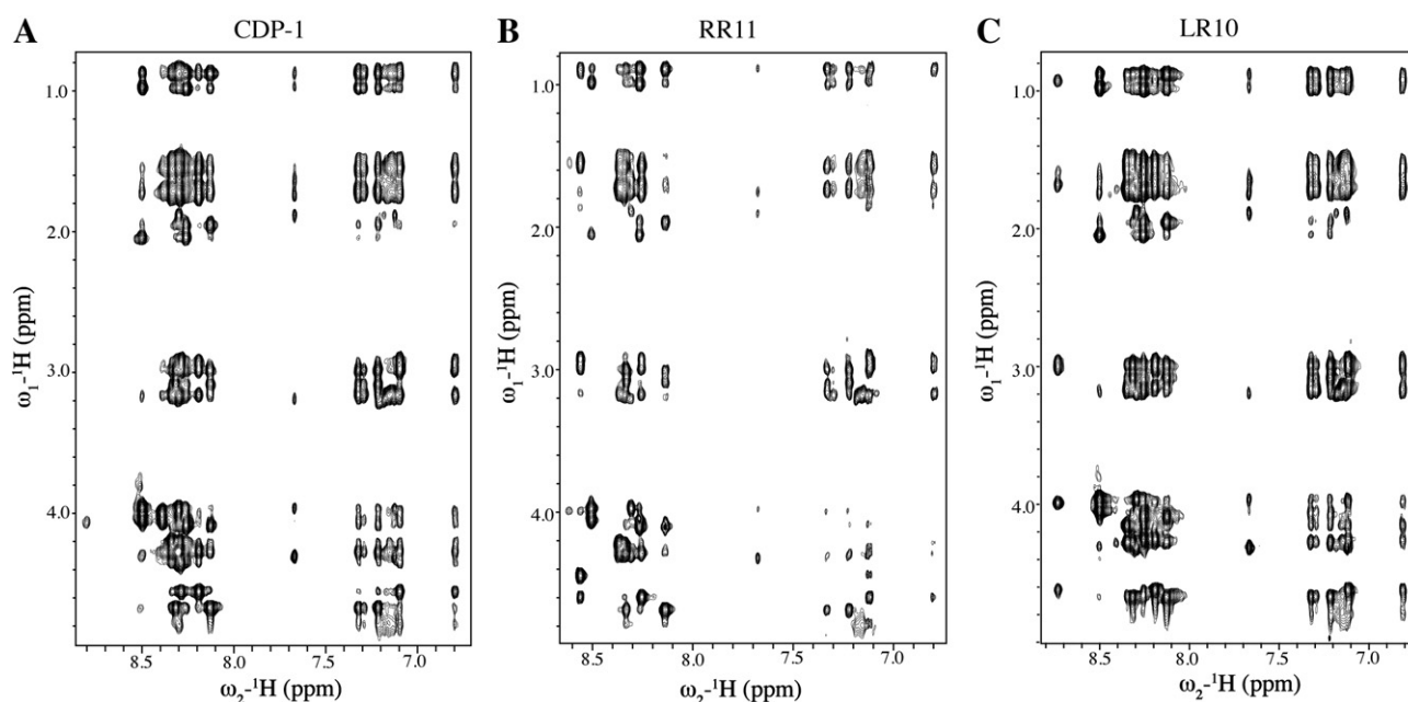
Fig. 5. Selected regions of the two-dimensional ^1\text{H} - ^1\text{H} tr-NOESY spectra of (A) CDP-1, (B) RR11 and (C) LR10 peptides in the presence of 50 \mu\text{M} LPS at 25 °C showing NOE cross-peaks involving low-field shifted ( \omega_2 - ^1\text{H} ) amide protons and aromatic sidechain protons resonances with up-field shifted ( \omega_1 - ^1\text{H} ) aliphatic proton resonances.
