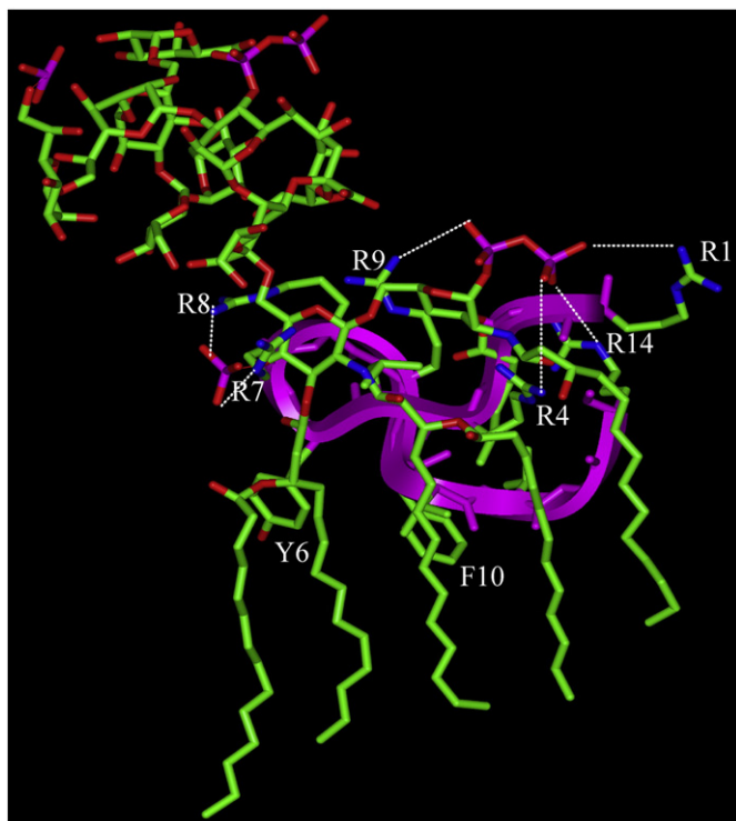
Fig. 9. A model of the complex of \beta -hairpin structure of CDP-1 with LPS showing plausible interactions and mode of binding. The complex may stabilize by ionic and/or hydrogen bond interactions among phosphate groups of the lipid A moiety with sidechains of basic residues of CDP-1. The acyl chains of LPS are in close proximity with the aromatic and nonpolar sidechains of residues of CDP-1. The model was constructed using INSIGHTII molecular modeling software.
