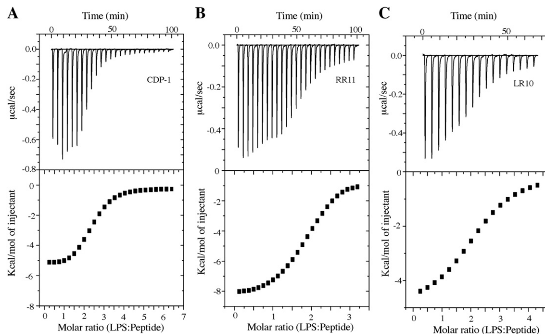
Fig. 2. (upper panels A–C) ITC thermograms of LPS binding to CDP-1, RR11 and LR10 peptides. (lower panels A–C) Plots showing molar ratios of LPS:peptides as a function of heat of binding. Data (lower panels A–C) represent best-fitted points according to one site binding mode. ITC experiments were carried out at 25 °C, 10 mM sodium phosphate buffer, pH 6.8.
