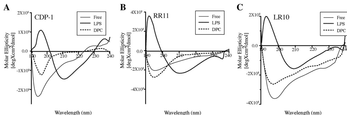
Fig. 4. Far UV CD spectra of CDP-1, RR11 and LR10 peptides in free aqueous solutions, solution containing LPS and solution containing DPC micelles. CD spectra were at 10 mM sodium phosphate buffer, pH 7.0.
