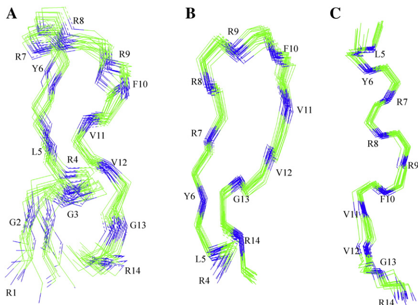
Fig. 7. Superposition of twenty lowest energy structures of (A) CDP-1, (B) RR11 and (C) LR10 peptides bound to LPS micelles determined using CYANA.
