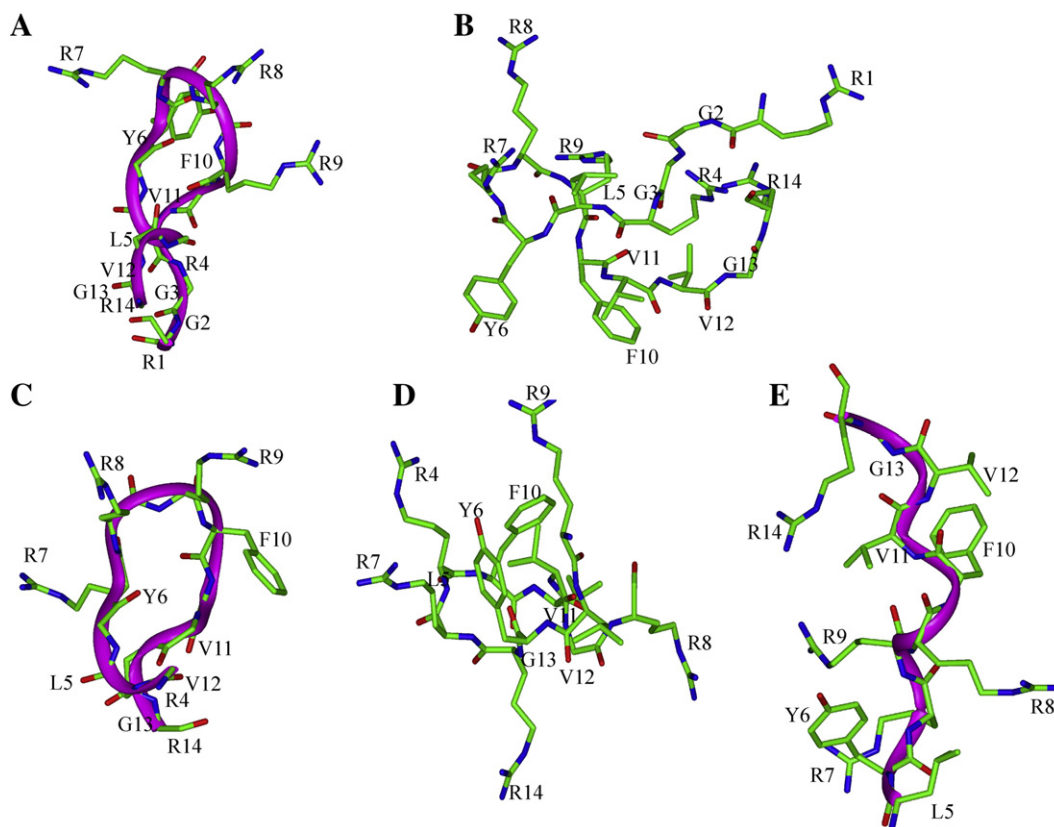
Fig. 8. Representative LPS bound structures and sidechain orientation topology of (A and B) CDP-1, (C and D) RR11 and (E) LR10 peptide.
