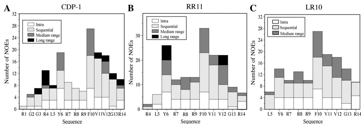
Fig. 6. Bar diagrams summarizing number and types (intra, sequential, medium-range and long-range) of NOEs of CDP-1, RR11 and LR10 peptides in complex with LPS used for structure determination.
